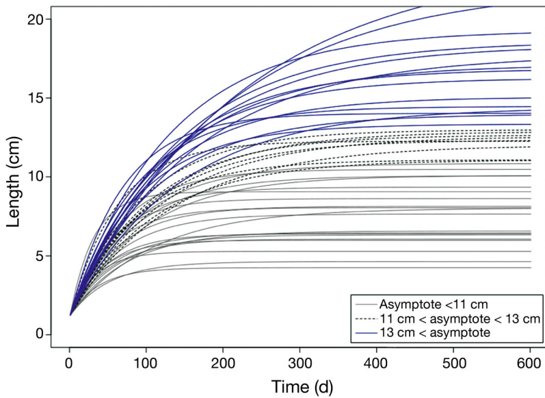
Fig. 3. Mirounga angustirostris . Growth trajectory of all whiskers of the captive elephant seal, showing high inter-whisker variation in curvature constant ( K ) and asymptotic whisker length ( L_{\infty} ) values. Coloring identifies whiskers with various ranges of asymptotic lengths
