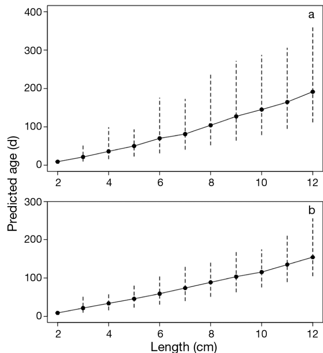
Fig. 4. Mirounga angustirostris . Predicted age as a function of size for (a) all whiskers and (b) 10 000 simulated whiskers at <75% of their asymptotic length. Black line: mean prediction; error bars: 95% confidence limits
