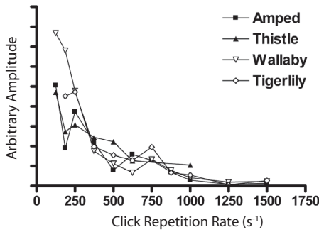
Figure 6. Relative amplitude of RFRs for four California sea lions when estimated as the square root of the sum power of the fundamental and harmonics up to 1,500 Hz.
