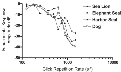
Figure 7. Amplitude of RFR fundamental as a function of click repetition rate in the California sea lion, northern elephant seal, Pacific harbor seal, and domestic dog; amplitudes are shown as dB re maximum fundamental response for each species. Data shown for the California sea lion are the average of the four subjects shown in Figure 5.
